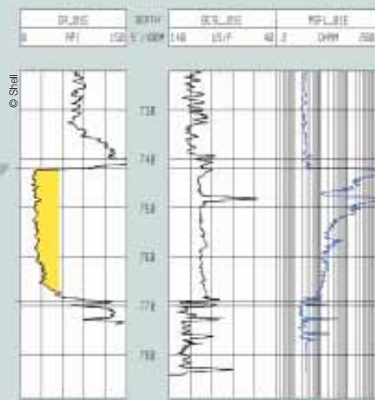
Example well log showing the reservoir horizon, the Lower Bentheim Sandstone.
